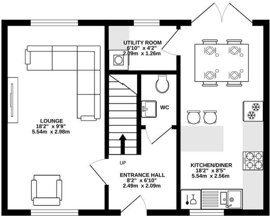
GROUND FLOOR 455 sq.ft. (42.3 sq.m.) approx.
